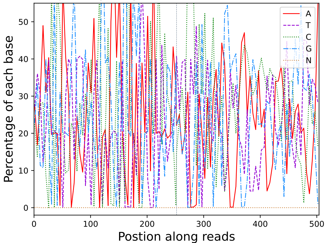
Base percentage along reads (R10122)
